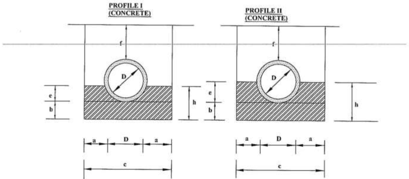
FIGURE C16-BEDDING AND HAUNCH PROFILE TYPES I & II
