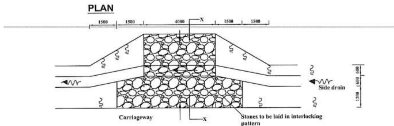
FIGURE C18-ACCESS DRIFT
