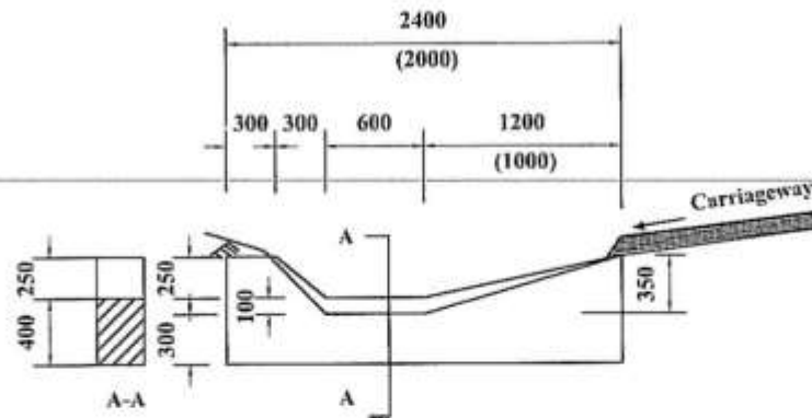
SECTION OF MASONRY SCOUR CHECK
