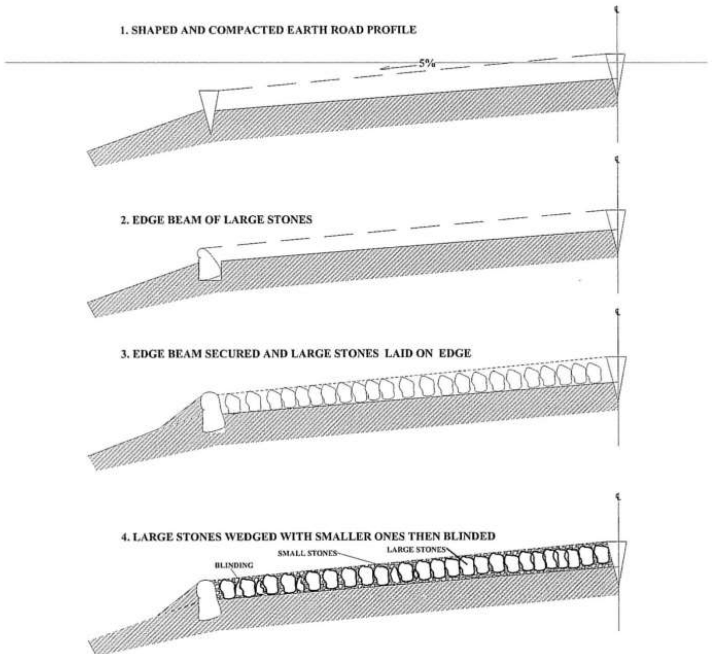
FIGURE C21-HAND PACKED STONE PAVEMENT
