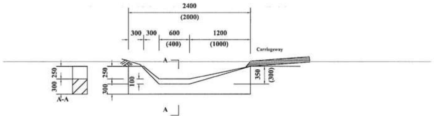
FIGURE C9b- CONCRETE SCOUR CHECKS
