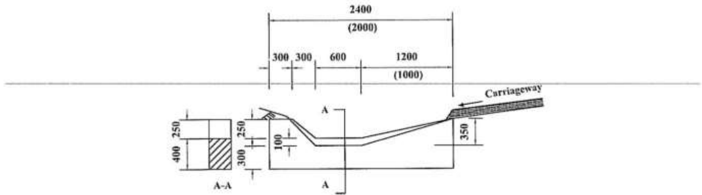
SECTION OF MASONRY SCOUR CHECK
