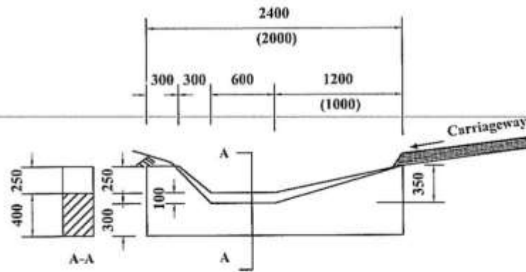
SECTION OF MASONRY SCOUR CHECK
