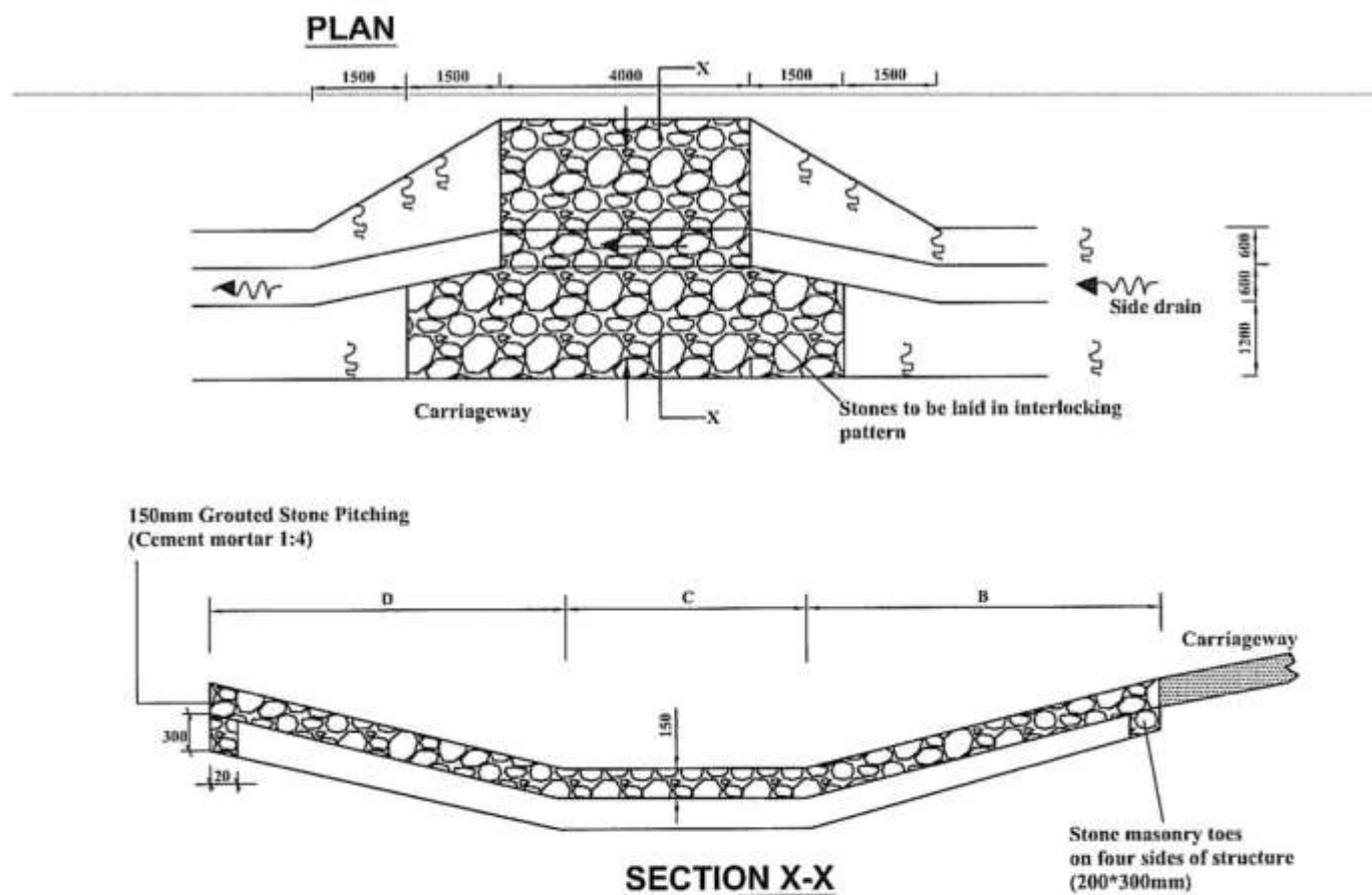
FIGURE C18-ACCESS DRIFT
